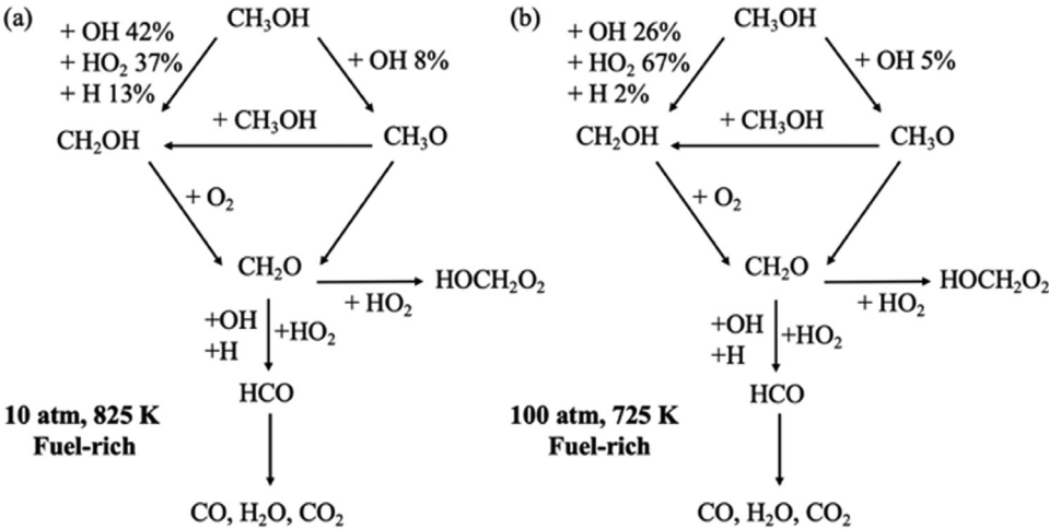
Fig. 3. Reaction pathways for onset of CH 3 OH oxidation at (a) 10 atm and (b) 100 atm using the updated HP-Mech model.
