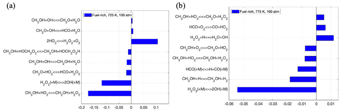
Fig. 4. Sensitivity analysis for CH 3 OH oxidation at (a) 725 K and (b) 775 K and 100 atm using updated HP-Mech model.
