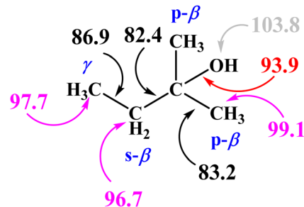
Fig. 1 Definitions of different carbon sites on 2-methyl-2-butanol (2M2B) with “p- \beta ” denoting the primary beta site and “s- \beta ” denoting the secondary beta site, and bond dissociation energies at 0 K ( \text{kcal mol}^{-1} ) calculated at the G4 41 level of theory.
