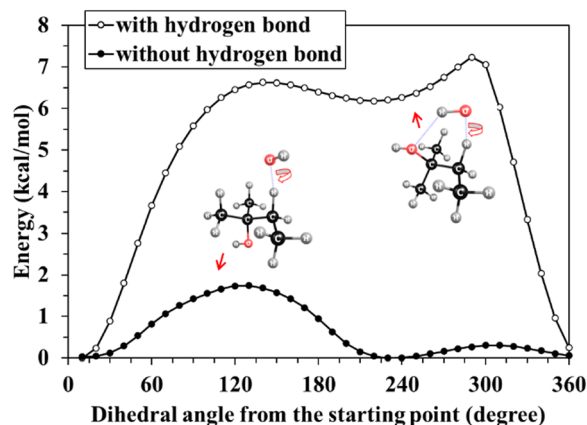
Fig. 3 Rotational potentials obtained at the M06-2X/6-31G level of theory for the same C-O torsional mode on the TS for the s-β H-atom abstraction reaction channel with and without hydrogen bonds, respectively.
