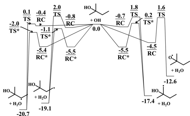
Fig. 2 ZPE corrected PESs (in units of \text{kcal mol}^{-1} ) for the H-atom abstraction reactions from 2M2B by \bullet\text{OH} at the QCISD(T)/CBS//M06-2X/6-311++G(d,p) level. “TS” denotes the transition state, “RC” denotes the van der Waals pre-reaction complex and asterisks mark the TSs with hydrogen bonds.
