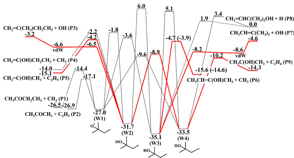
Fig. 9 ZPE corrected PESs (in units of \text{kcal mol}^{-1} ) for the unimolecular isomerization and \beta -scission reactions of 2M2B radicals at the QCISD(T)/CBS//M06-2X/6-311++G(d,p) level (with important reaction channels in red). The relative energies for W3 = P6 ( cis ) are in parentheses.
