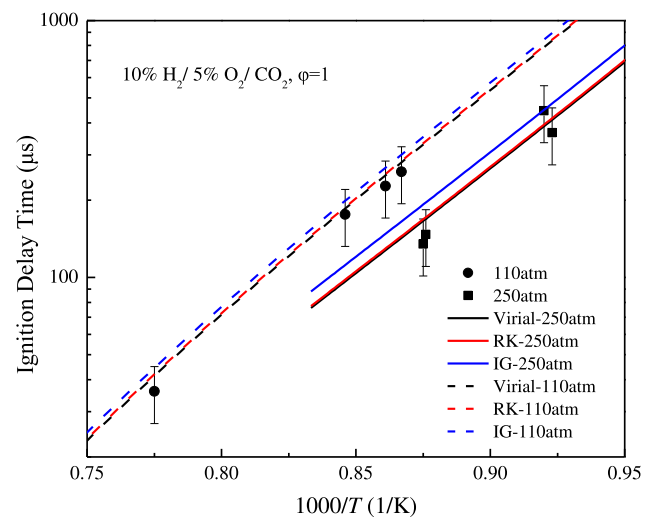
Fig. 13. The ignition delay time modeling for H_2 oxidation in carbon dioxide and comparison with experimental data [39].
