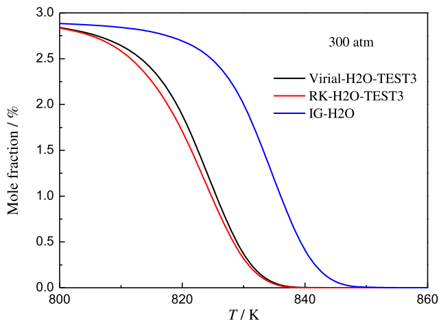
Fig. 6. Mole fraction of H_2 verse temperature at 300 atm in the adiabatic flow reactor simulation by using Virial EoS-TEST3, RK-TEST3, and ideal-gas EoS. TEST3: chemical potentials only. H_2:O_2:H_2O = 2.9:4.24:92.86 . Residence time = 295 \text{ K} \cdot 0.6 \text{ s} / T .
