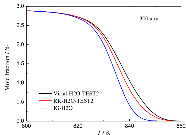
Fig. 5. Mole fraction of H_2 verse temperature at 300 atm in the adiabatic flow reactor simulation by using Virial-TEST2, RK-TEST2, and ideal-gas EoS. TEST2:real-fluid thermodynamic properties only. H_2:O_2:H_2O = 2.9:4.24:92.86 . Residence time = 295\text{ K} \cdot 0.6\text{ s} / T .
