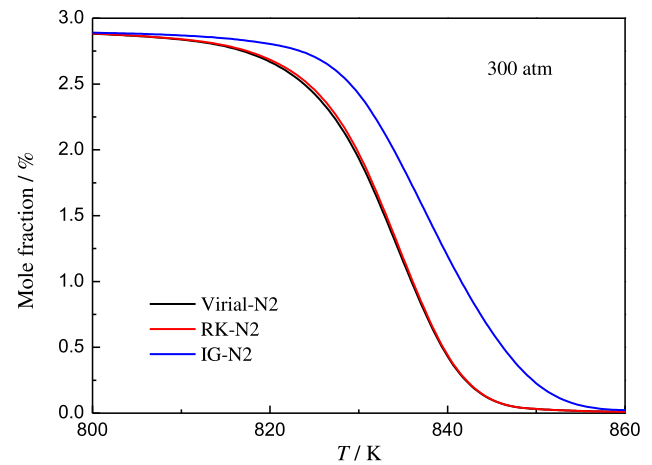
Fig. 8. Mole fraction of H_2 verse temperature at 300 atm in the adiabatic flow reactor simulation by using Virial, RK, and ideal-gas EoS. H_2:O_2:H_2O = 2.9:4.24:92.86 . Residence time = 295 \text{ K} \cdot 0.6 \text{ s} / T .
