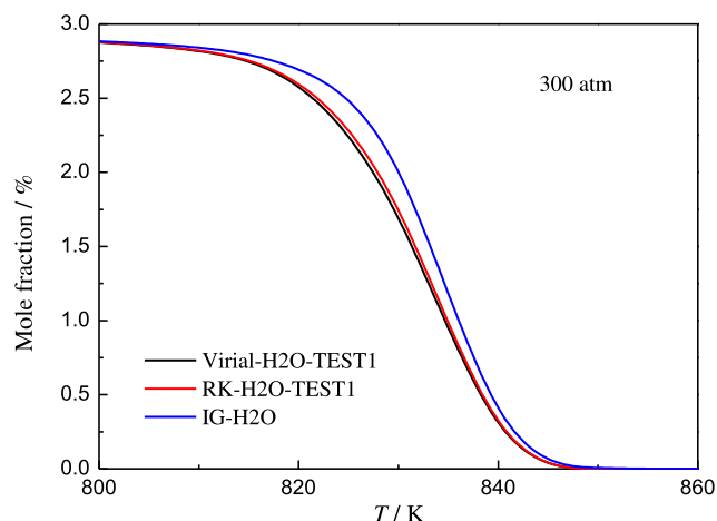
Fig. 4. Mole fraction of H_2 verse temperature at 300 atm in the adiabatic flow reactor simulation by using Virial-TEST1, RK-TEST1, and ideal-gas EoS. TEST1:real-fluid EoS only. H_2:O_2:H_2O = 2.9:4.24:92.86 . Residence time = 295\text{ K} \cdot 0.6\text{ s} / T .
